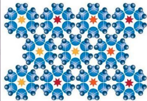
Pollutants held within hexagonal structures
